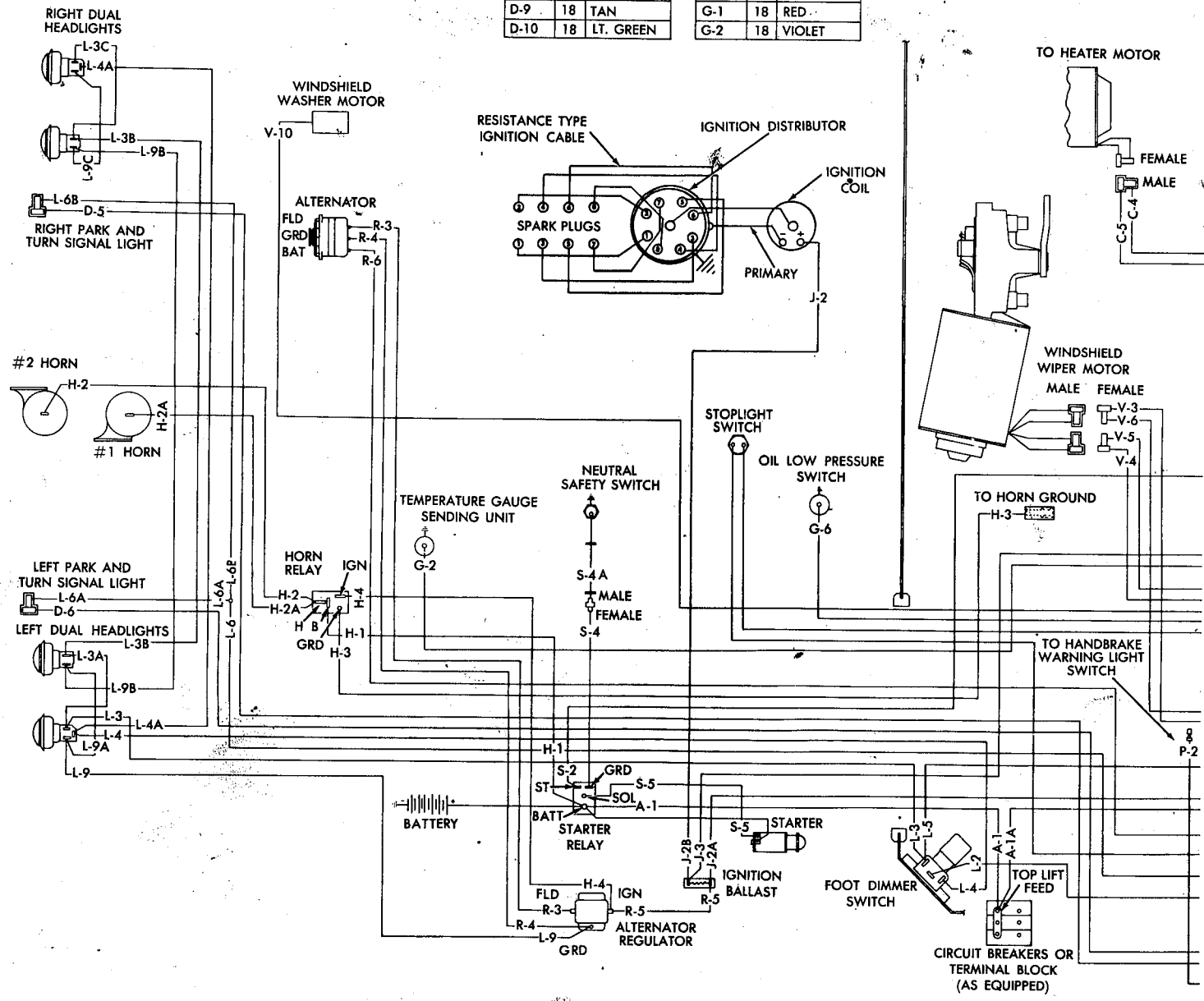
Fig. 64—Chassis and Instrument Panel Wiring Diagram (Chrysler)
