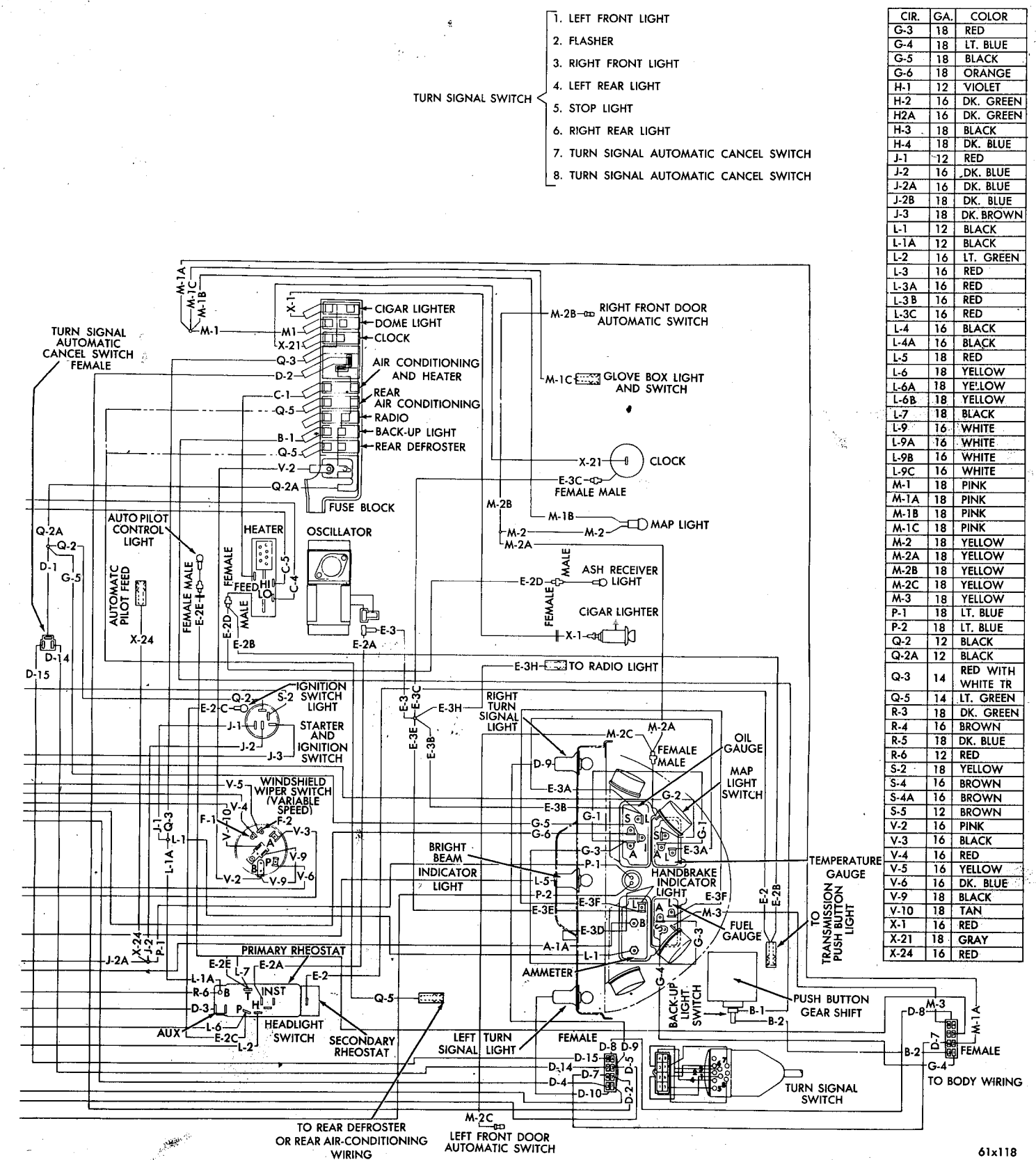
Fig. 64—Chassis and Instrument Panel Wiring Diagram (Chrysler)
